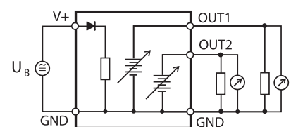
Schematic 3-wire type (voltage signal)
